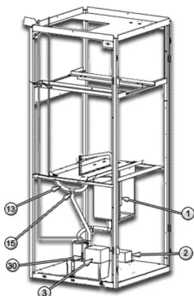
A: UpFlow Steam Generating Humidifier Option w/ Condensate Pump
