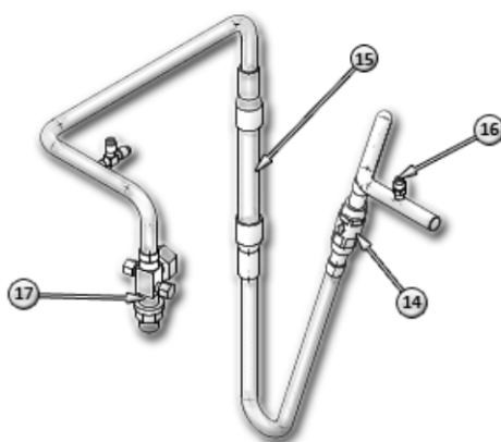
DISCHARGE ASSY CR020RW
