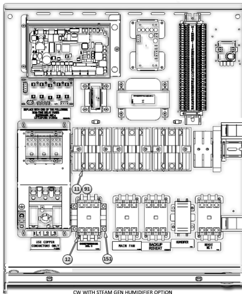
CW WITH STEAM GEN HUMIDIFIER OPTION
