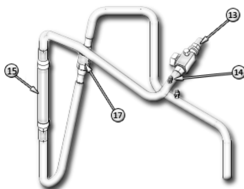
DISCHARGE BOTTOM ASSY CR020/CR035
