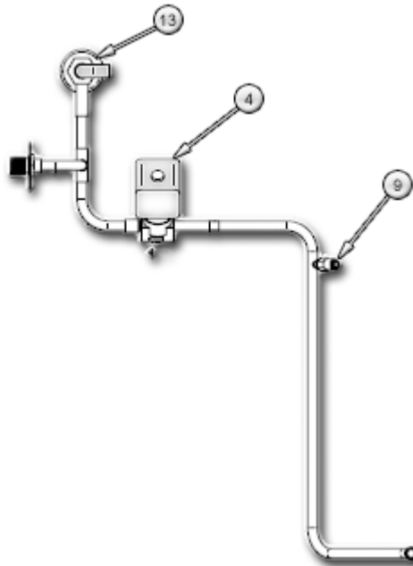
LIQUID ASSEMBLY
