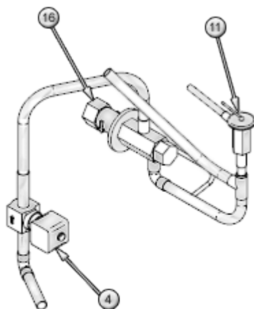
HGBP/LIV ASSEMBLY
